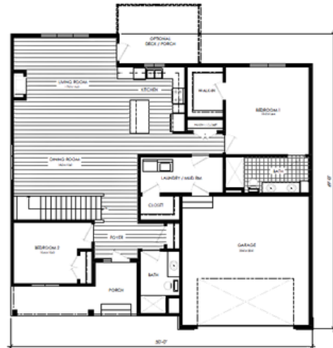
Henry: 1,627 SQ FT Main Floor
