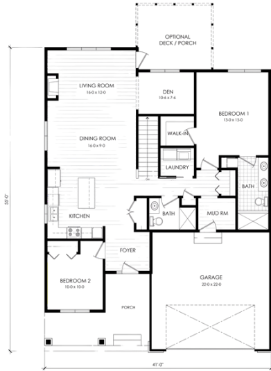
Stewart: 1,500 SQ FT Main Floor
